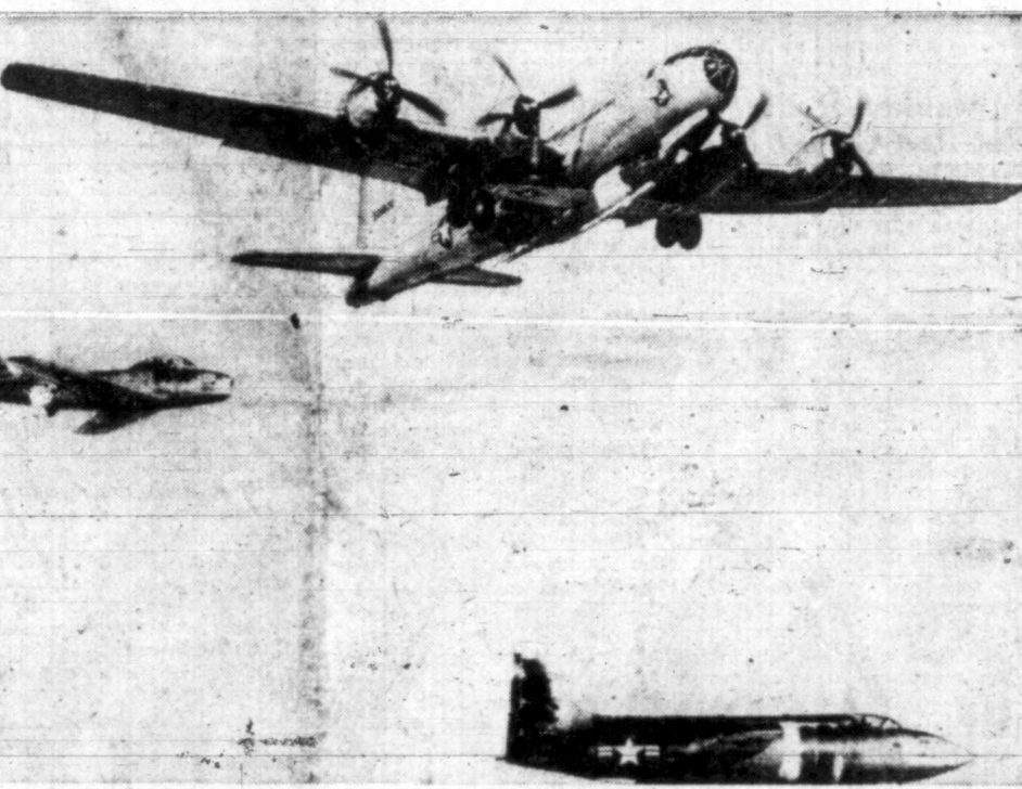
NEWEST ROCKET-POWER research plane is the Bell X-1A, shown (upper) carried aloft by a B-29 at Edwards Air Force Base, Calif., and (lower right) swooshing along on its first powered flight, in front of an F-86 "chase" plane used to keep a close check on the X-1A's performance.
