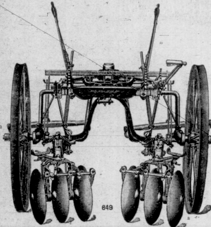
P. & O. Wiggletail Disc Cultivator
