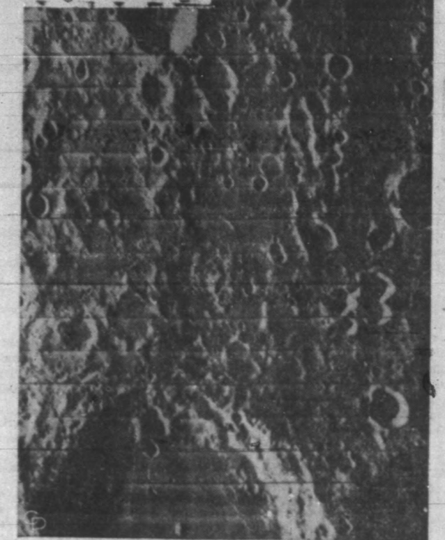
LUNAR ORBITER 5 sends back this photo of the far side of the Moon never photographed before. It is about 90 miles by 120 miles, in the area of Mare Orientale.
